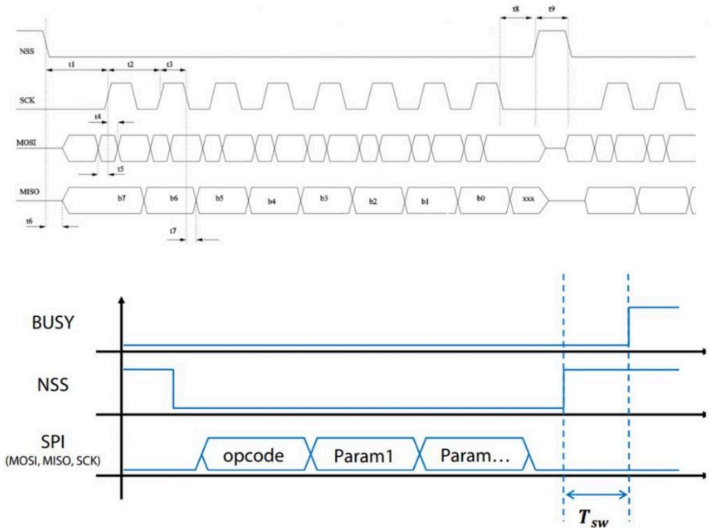
Figure 8-3: Switching Time Definition
